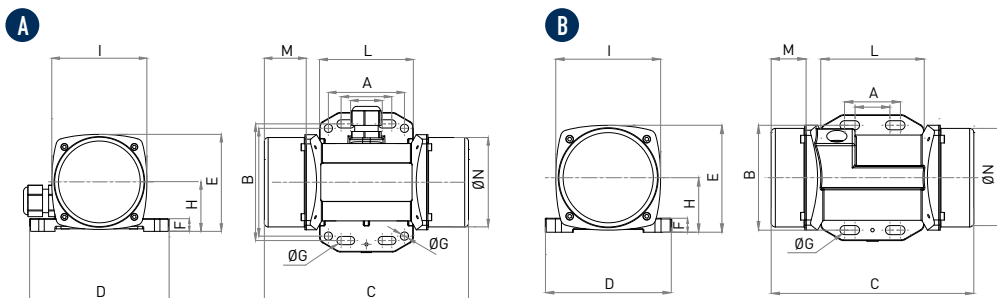
DIMENSIONAL SPECIFICATIONS
